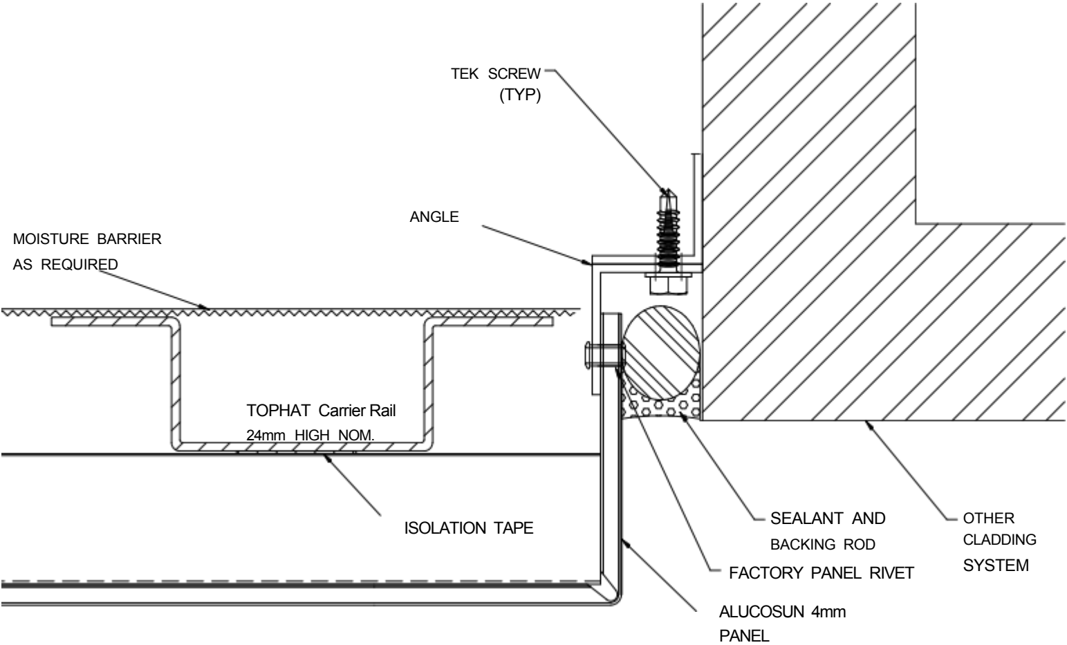
7. WALL ABUTMENT DETAIL
